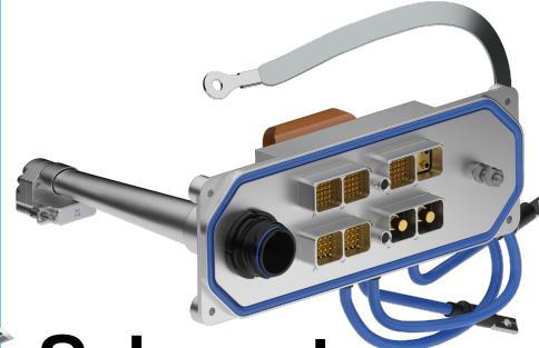
Sub-system integration
